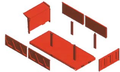
Ribaltabile Trilaterale Three-Way Tipper
